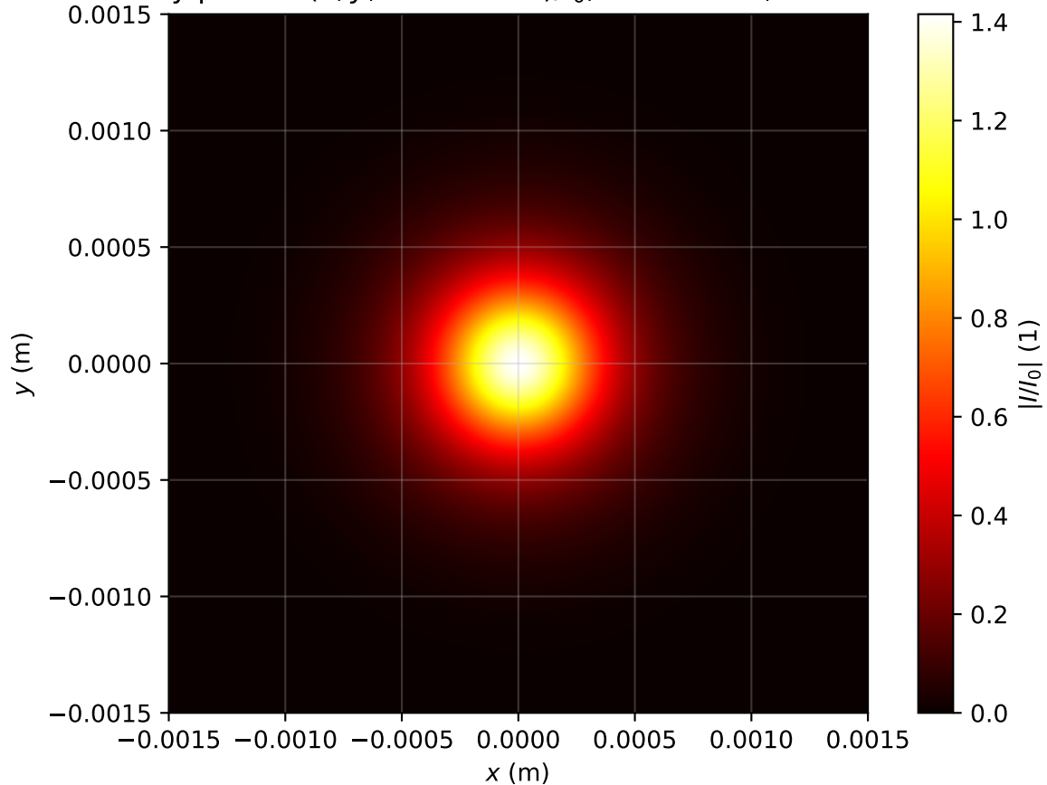
Intensity profile I(x, y, z = 1.035m)/I_0 , Pin=0.9Pcr, artificial time
